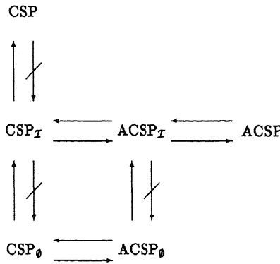
Figure 4: The CSP-ACSP hierarchy.
